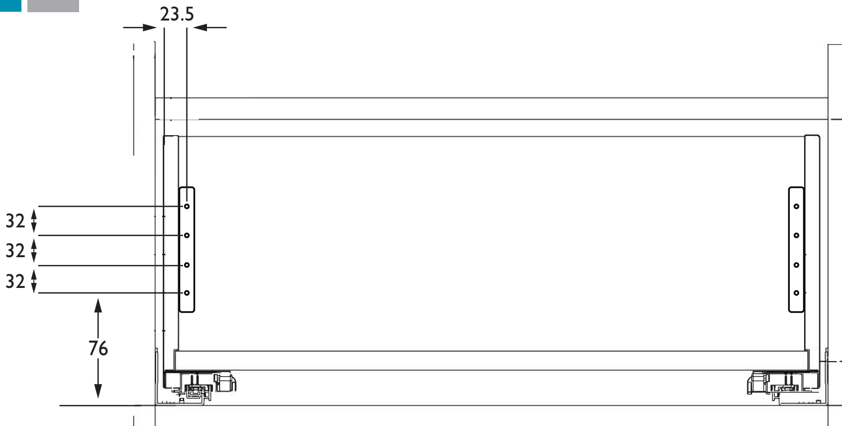
REAR PANEL DRILLING HOLES
