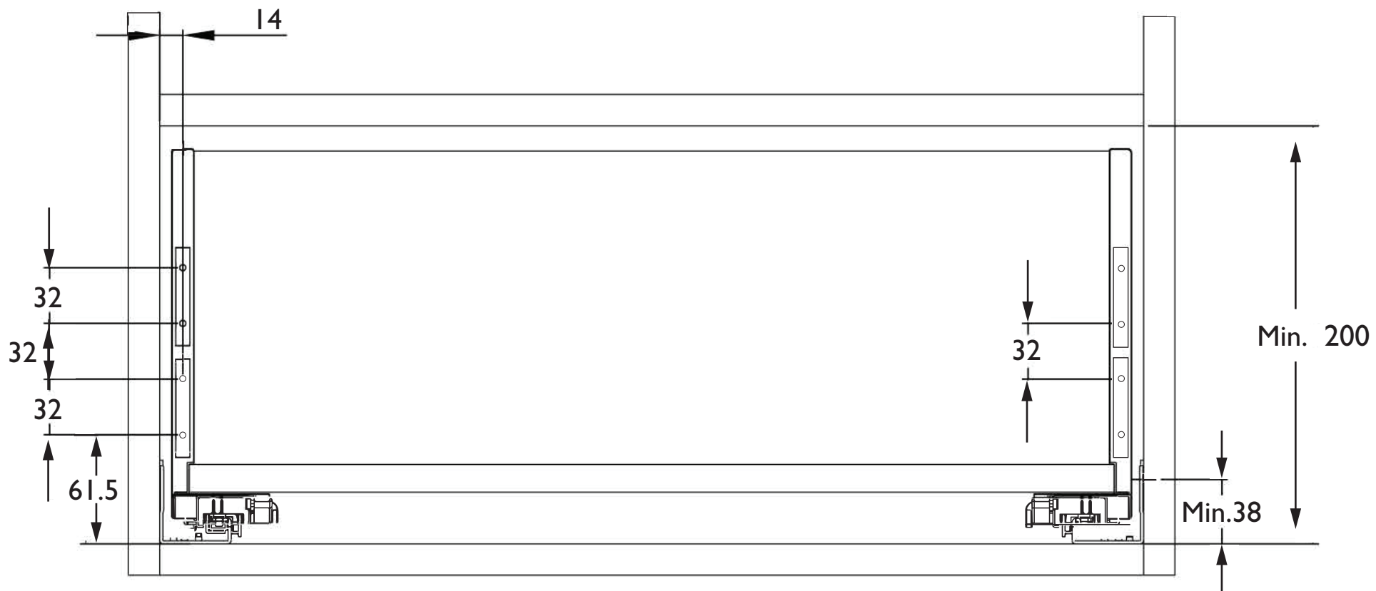
FRONT BRACKET DRILLING HOLES
