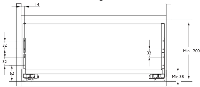
ENKO SLIMBOX 180mm High
